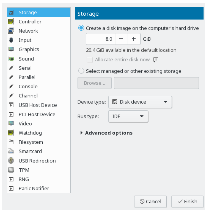
FIGURE 14.9: ADD A NEW STORAGE
