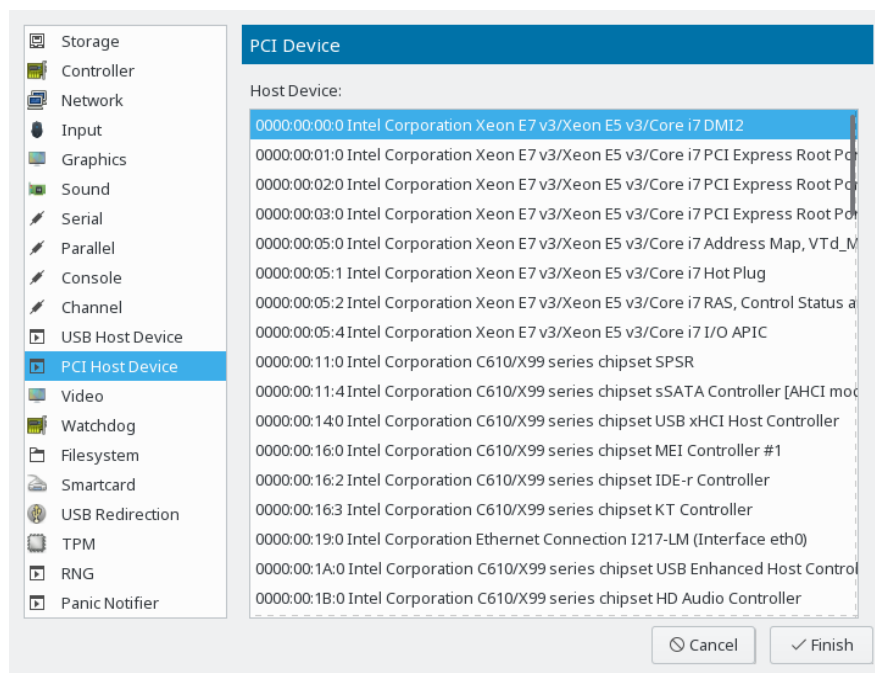
FIGURE 14.12: ADDING A PCI DEVICE
